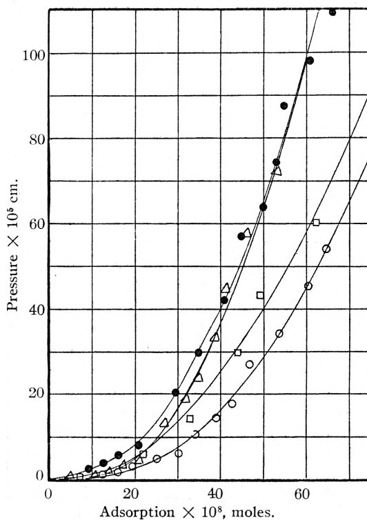
Fig. 3.—Adsorption of nitrogen on glass spheres activated at room temperature: ○, Run 1; □, Run 3; △, Run 4; ●, Run 5.
