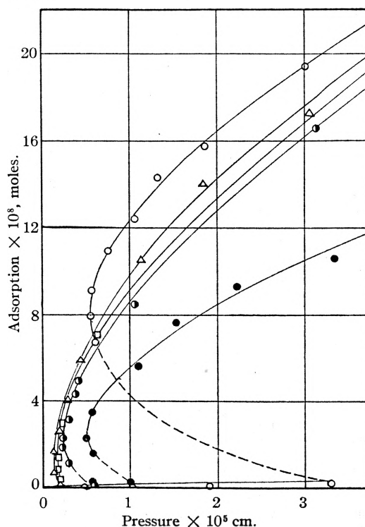
Fig. 5.—Adsorption of nitrogen at low pressures on glass spheres activated at room temperature: ○, Run 1; ●, Run 2; □, Run 3; △, Run 4; ●, Run 5.
